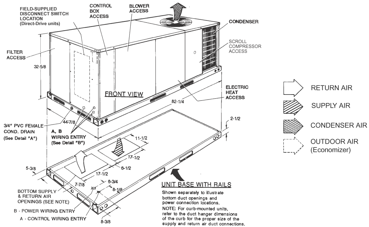
Figure 5: XP036-060 Heat Pump/Electric Heat Front View Physical Dimensions
