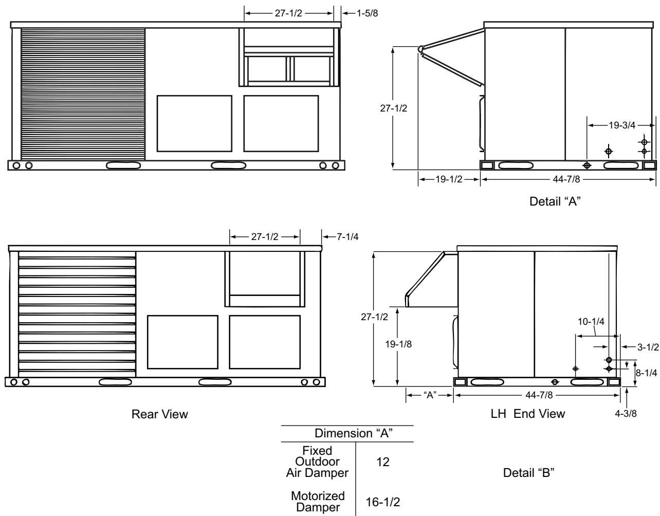
Figure 6: XP036-060 Fixed Outdoor Air Motorized Damper Rain Hood Physical Dimensions
