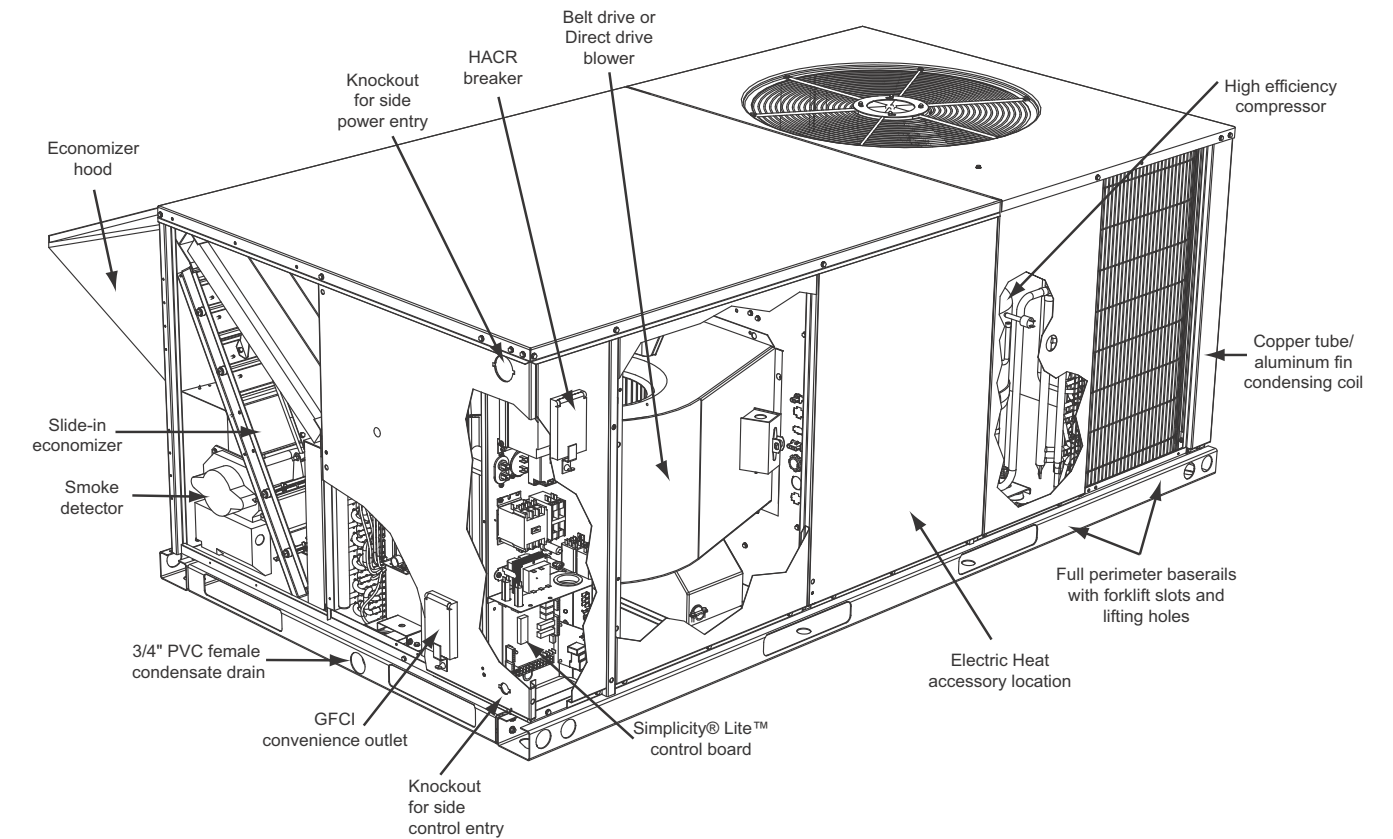
Figure 1: XP036-060 Component Location
