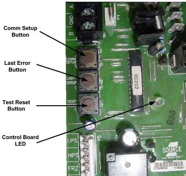
Figure 18: Unit Control Board
