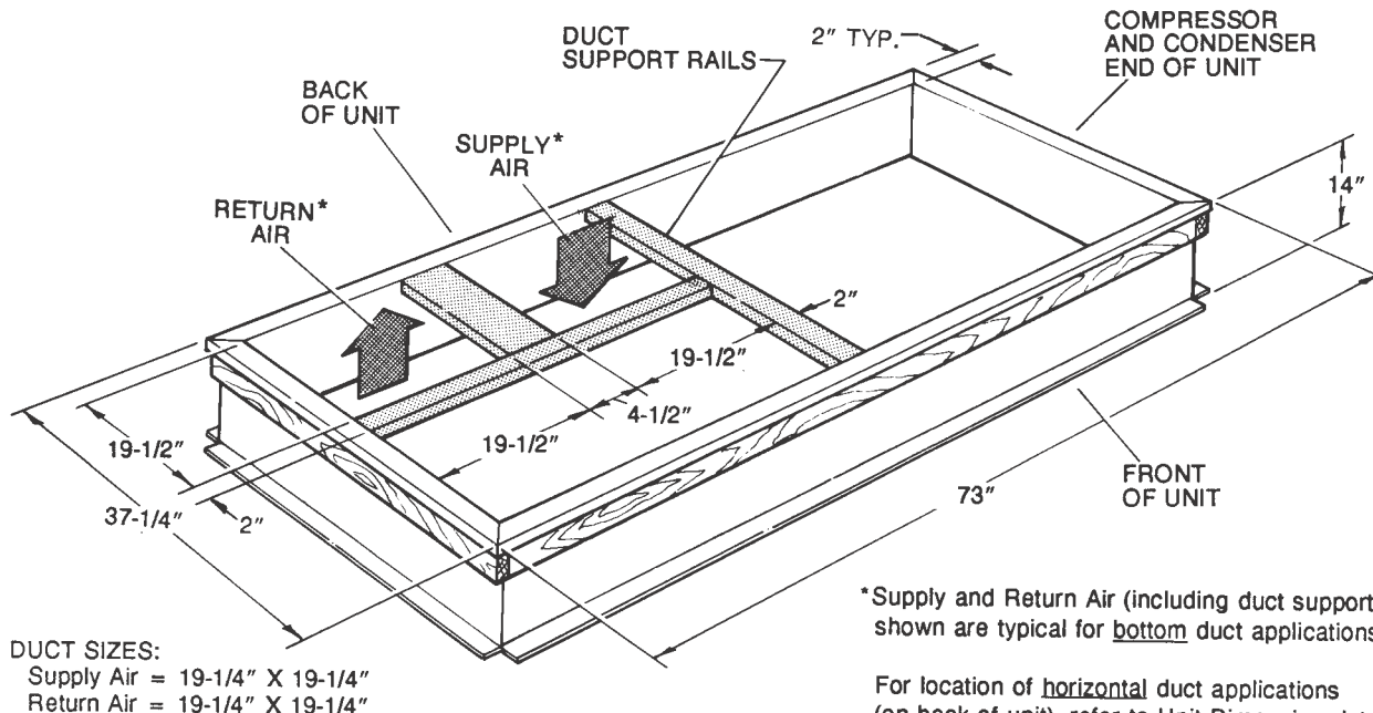
Figure 9: XP036-060 Roof Curb
