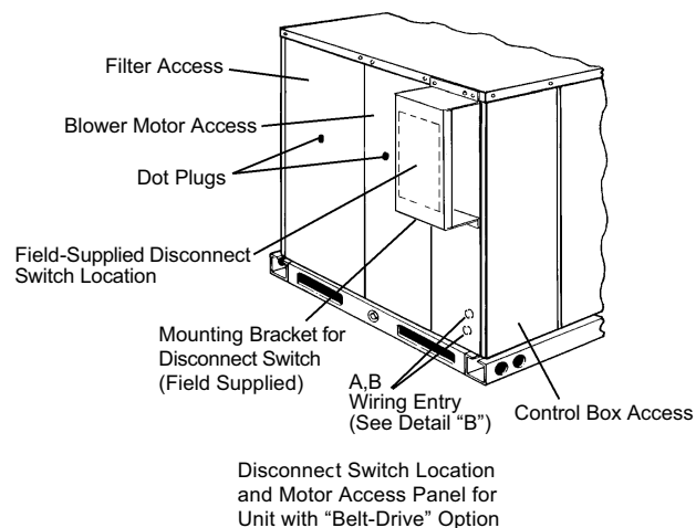
Figure 7: XP036-060 Disconnect Location
