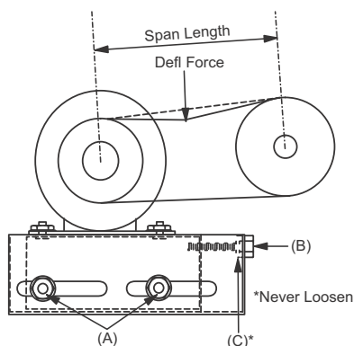
Figure 15: Belt Adjustment
