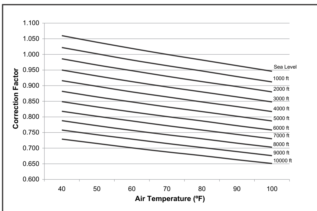
Figure 16: Altitude/Temperature Correction Factors
