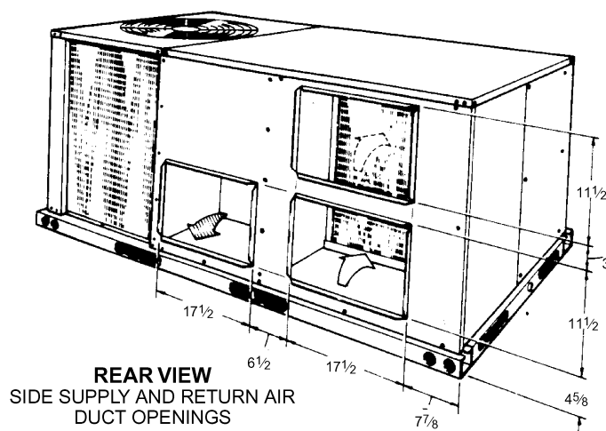
Figure 8: XP036-060 Unit Side Duct Openings
